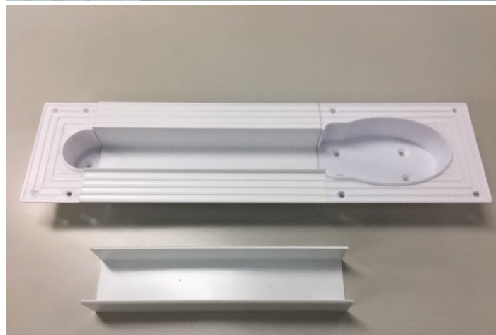
Sample with SRB1F, RT1F and SMB1F. Bendable track RT1B sample.
